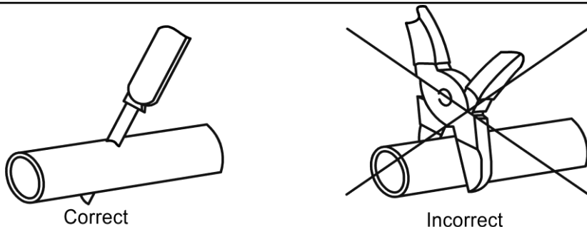
Figure 7.9 – Cutting the fuel pipe before installation
