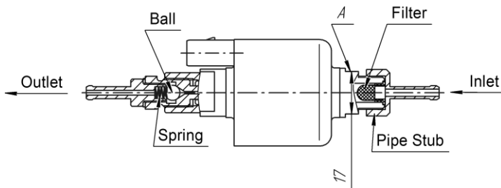
Figure 9.1 – Fuel pump
