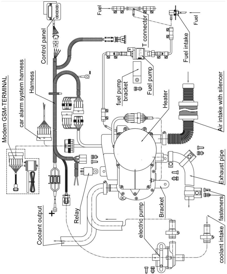
Figure 4.2 – Pre-heater basic components
